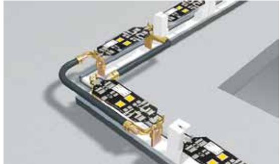
COS-4A Corner bridging with 1x8cm + 1x11cm conductors of 2.5mm 2
