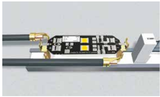
COS-3 Power connector with 2x1m conductors of 2.5mm 2
